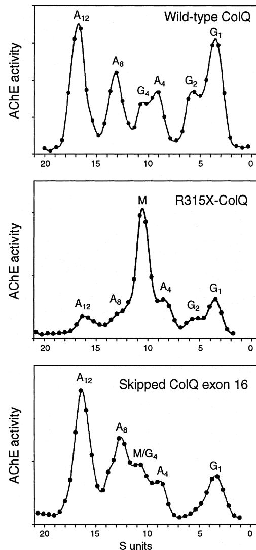
Figure 7 Sedimentation profiles of AChE species extracted from COS cells transfected with the indicated COLQ cDNA along with the wild-type ACHE T cDNA. G_1 , G_2 , and G_4 are globular forms; A_4 , A_8 , and A_{12} are asymmetric forms; M is a \sim 10.5 S mutant peak composed of a catalytic tetramer bound to a truncated single strand of ColQ.
